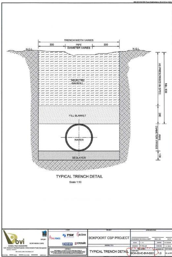
Figure 1 – Profile of the proposed pipeline trench
