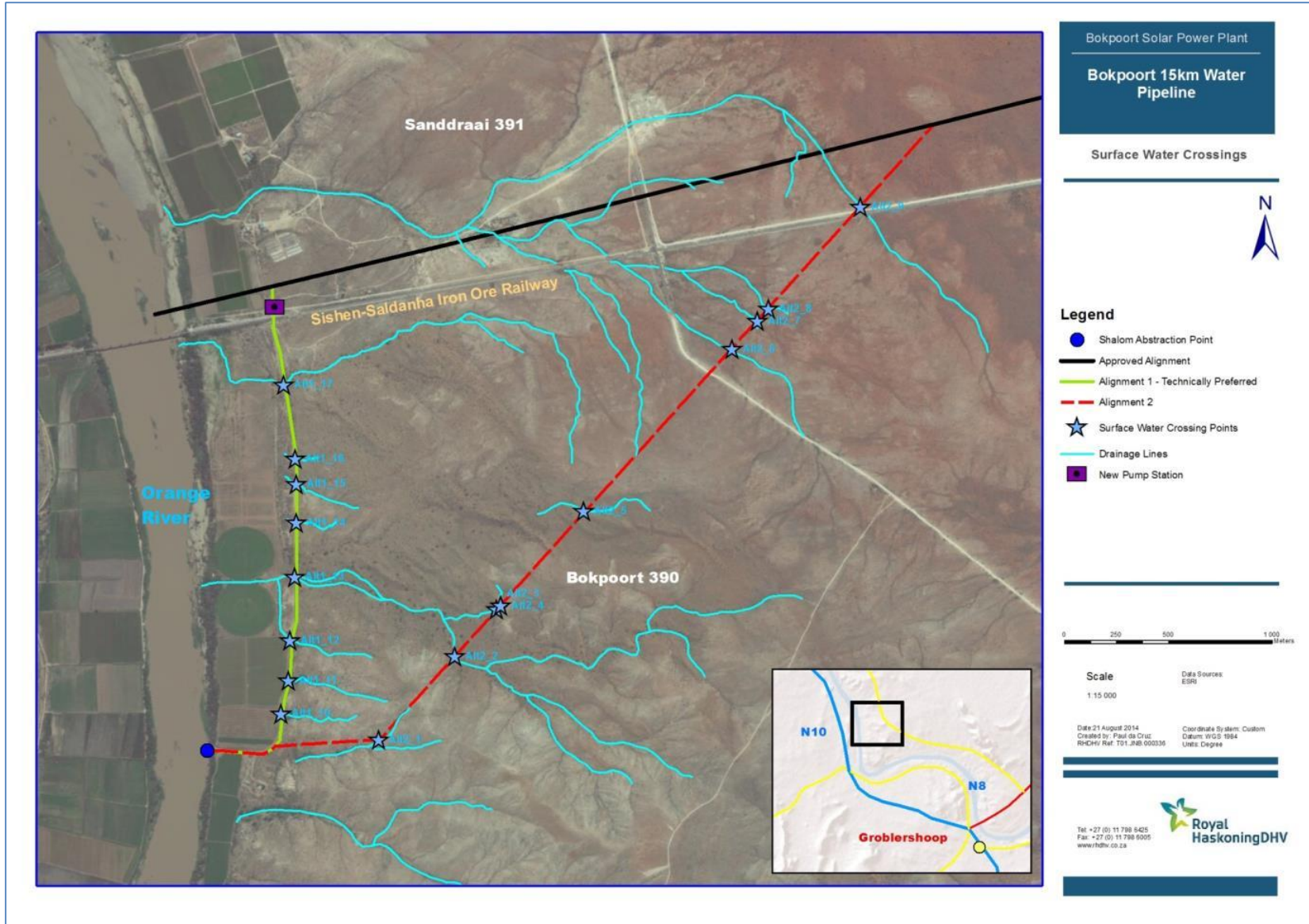
Figure 6 – Surface water drainage on the study site and location of surface water crossings along the two alternative alignments
