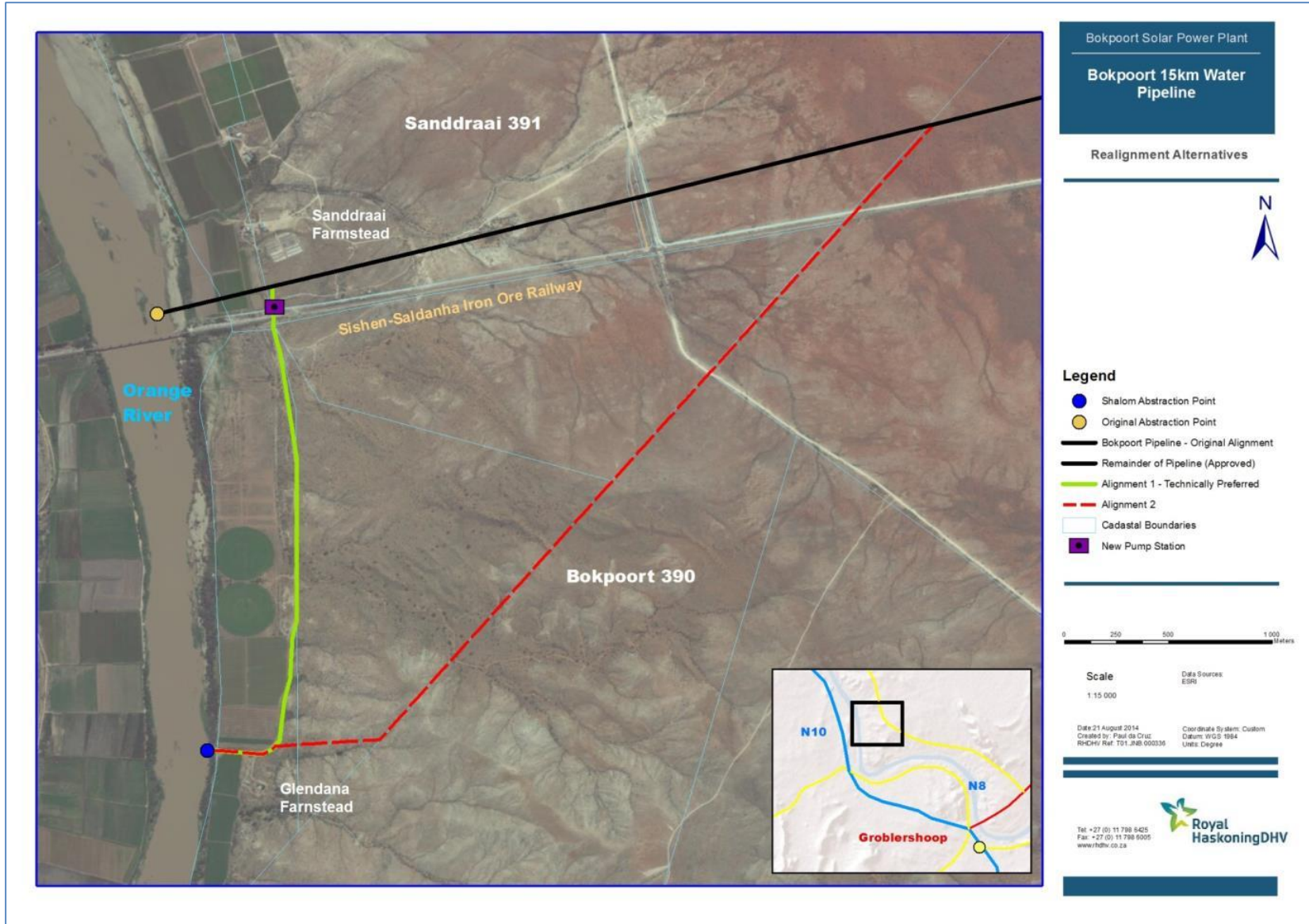
Figure 3 – Realigned Pipeline Alternatives
